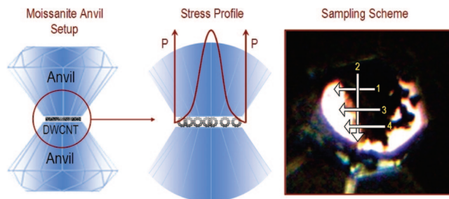
Figure 2. Scheme of the experimental setup, stress distribution inside the cell, and photograph of the sample under uniaxial conditions. The paths labeled in the photograph correspond to the four experimental runs described in the text.
