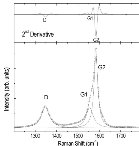
Figure 4. Band analysis for D and G modes of DWCNTs. The Raman spectrum shown in the figure was measured at 4 \text{ cm}^{-1} resolution at room conditions.
